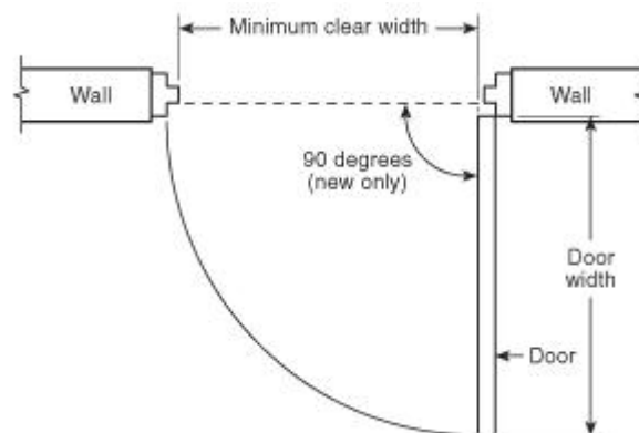
FIGURE A.7.2.1.2.3(a) Minimum Clear Width.
