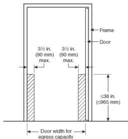
FIGURE A.7.2.1.2.1(a) Door Width — Egress Capacity.
