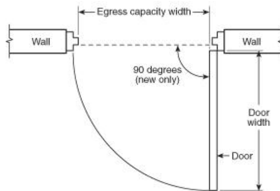
FIGURE A.7.2.1.2.1(a) Door Width — Egress Capacity.
