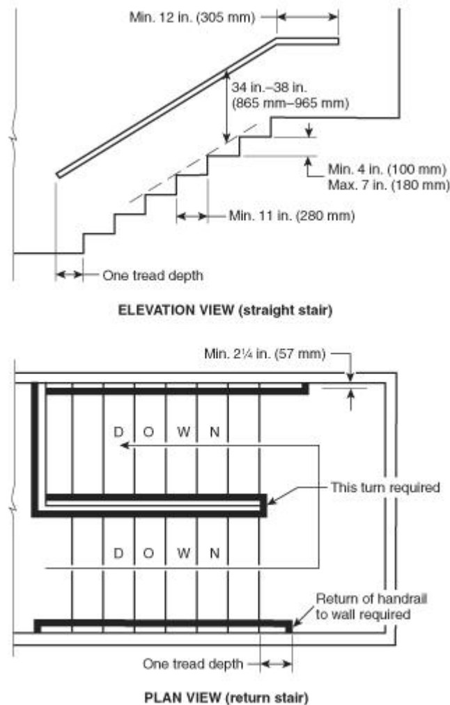
FIGURE A.7.2.2.4.4 Handrail Details.
